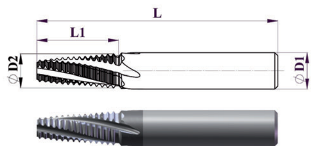
STANDARD TAPER – HELICAL FLUTES
