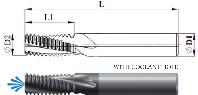
HELICAL FLUTES WITH COOLANT – UPON REQUEST
